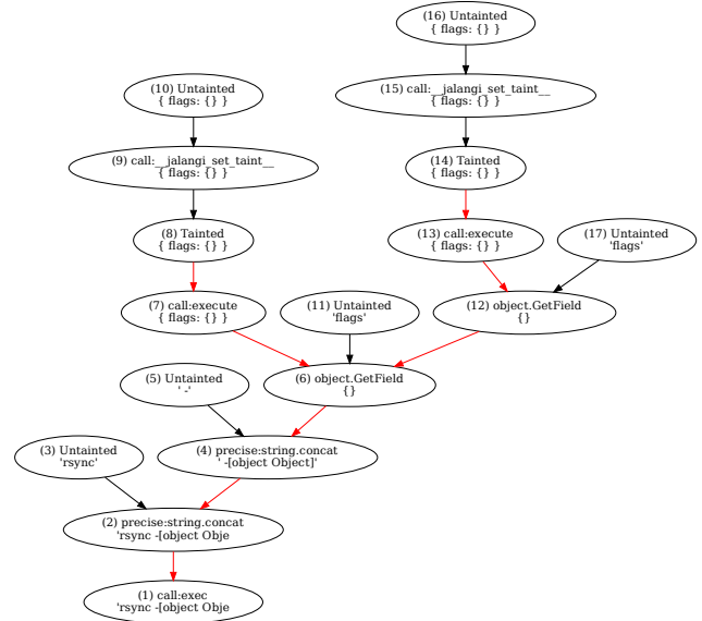
Fig. 3: Example provenance graph for code in Figure 2
