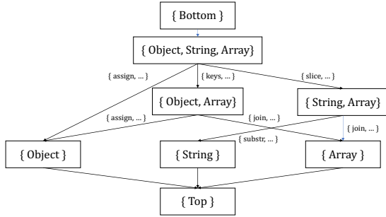
Fig. 7: Type lattice for object, string, and array types. Only a subset of edge labels are included for readability.
