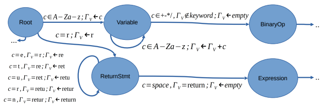
Fig. 11: A section of the graph representation of JavaScript syntax used by the Enumerator. Edges have labels C;U where C is a condition over the current character in the prefix c and the context \Gamma_V . U is a context update.
