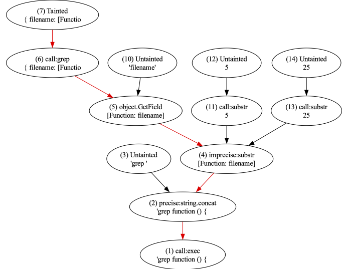
Fig. 5: Provenance graph for toy example API.
