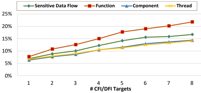
Figure 8: Runtime overhead incurred by the CFI/DFI enforcement with an increasing number of control transfer and data access targets to validate ( N=[1..8] ).
