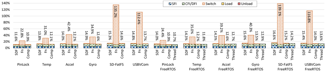
Figure 6: The runtime overhead of bare-metal and RTOS applications with different compartment units. CFI/DFI enforcement is enabled in all compartmentalization techniques with one target validated at every shared and peripheral data access (N=1).
