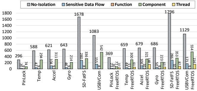
Figure 5: Average number of ROP gadgets per compartment.
