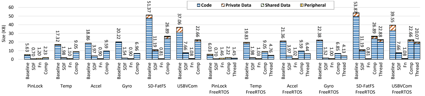
Figure 4: Average size of secure-world address space accessible by no-intra-TEE isolation firmware and compartments based on different compartment units: sensitive data flow (SDF), function (Fn), component (Comp), and thread (Thread).
