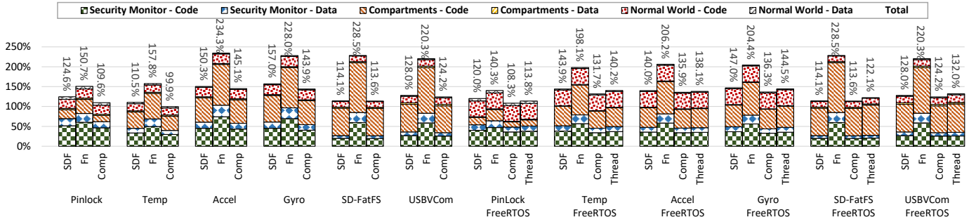
Figure 7: Memory footprint of sensitive data protection using different compartmentalization techniques (size is normalized to the unprotected firmware).
