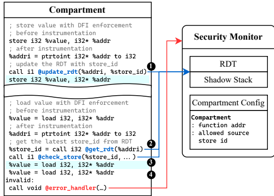
(b) CFI and DFI enforcement.
