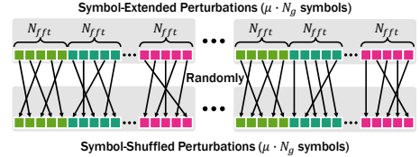
Fig. 5: Symbol shuffling mechanism. The complex-valued symbols assigned to the subcarriers are randomly shuffled.
