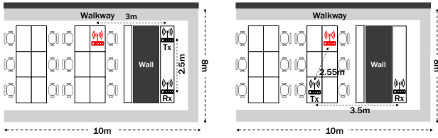
(a) LoS Tx/Rx path (b) NLoS Tx/Rx path Fig. 6: Experimental settings established in Magmaw.
