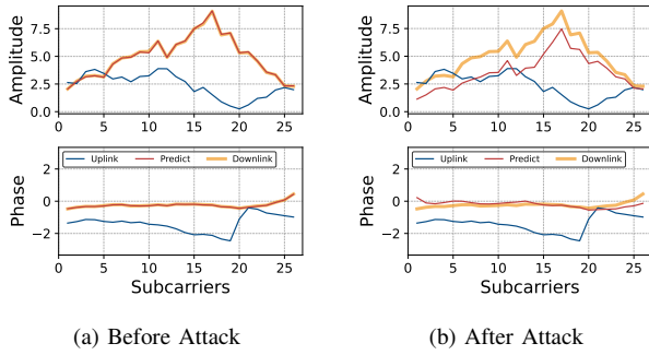
Fig. 19: Attack results on FIRE [54]. We visualize the channel amplitude and phase. FIRE takes the uplink channel (blue line) as input and predicts the downlink channel (red line) that is expected to be the same as the ground truth (yellow line).
