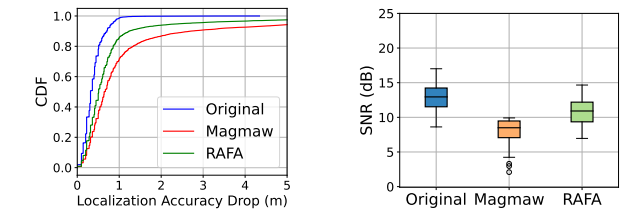
Fig. 18: Attack results on CSI-based models (PSR is -12dB).
