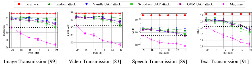
Fig. 7: Magmaw on ML-based wireless communication systems (i.e., modality-specific JSCC models).
