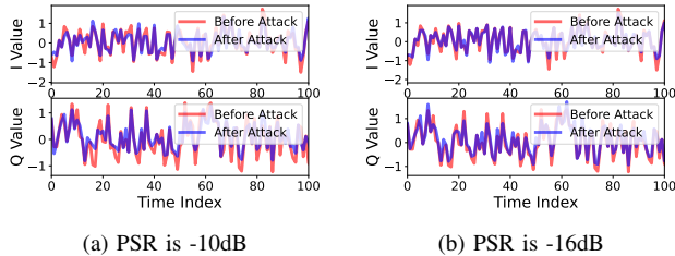
Fig. 9: Effect of perturbation when modulation is 16-QAM.
