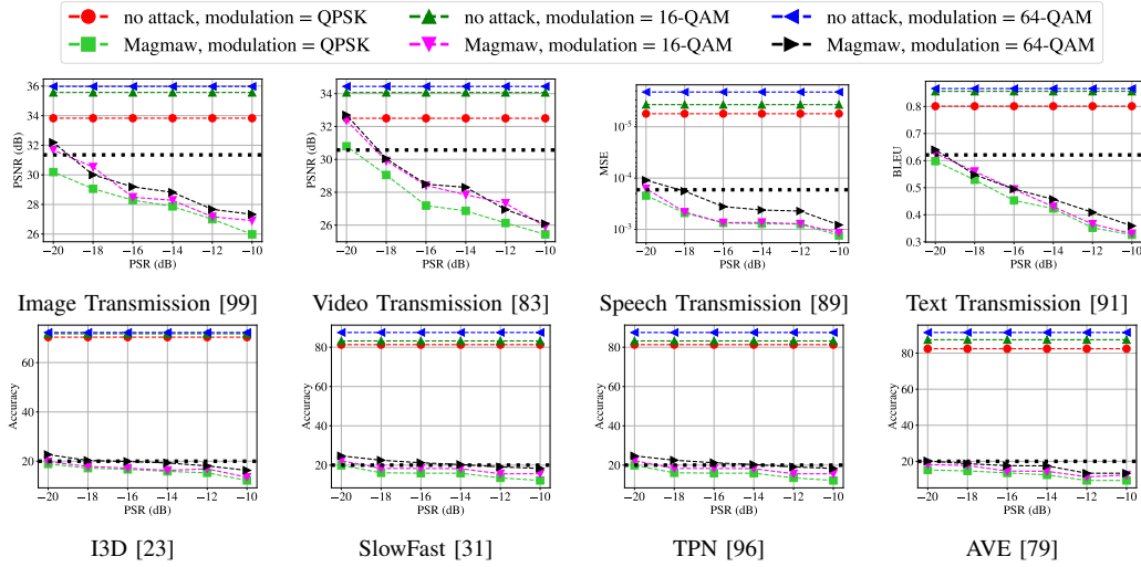
Fig. 20: Magmaw on wireless systems with different types of constellation mapping schemes (i.e., QPSK, 16-QAM, 64-QAM). The first and second rows are the results of JSCC and downstream tasks, respectively.
